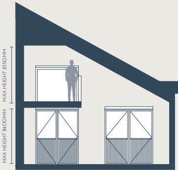
MEZZANINE ELEVATION
